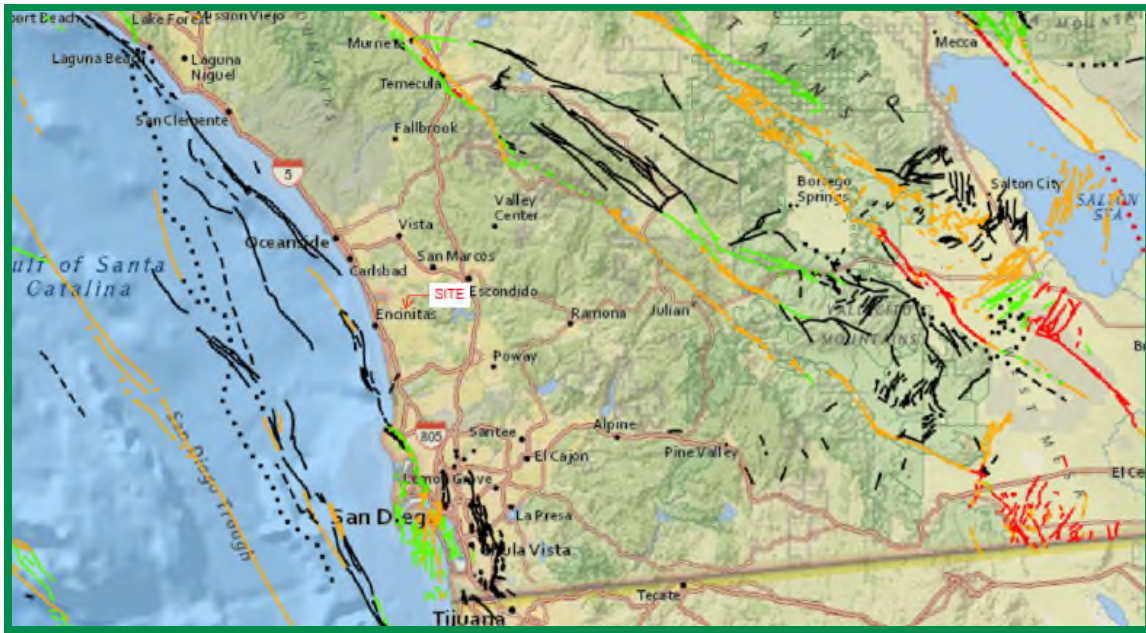
Faults in Southern California
