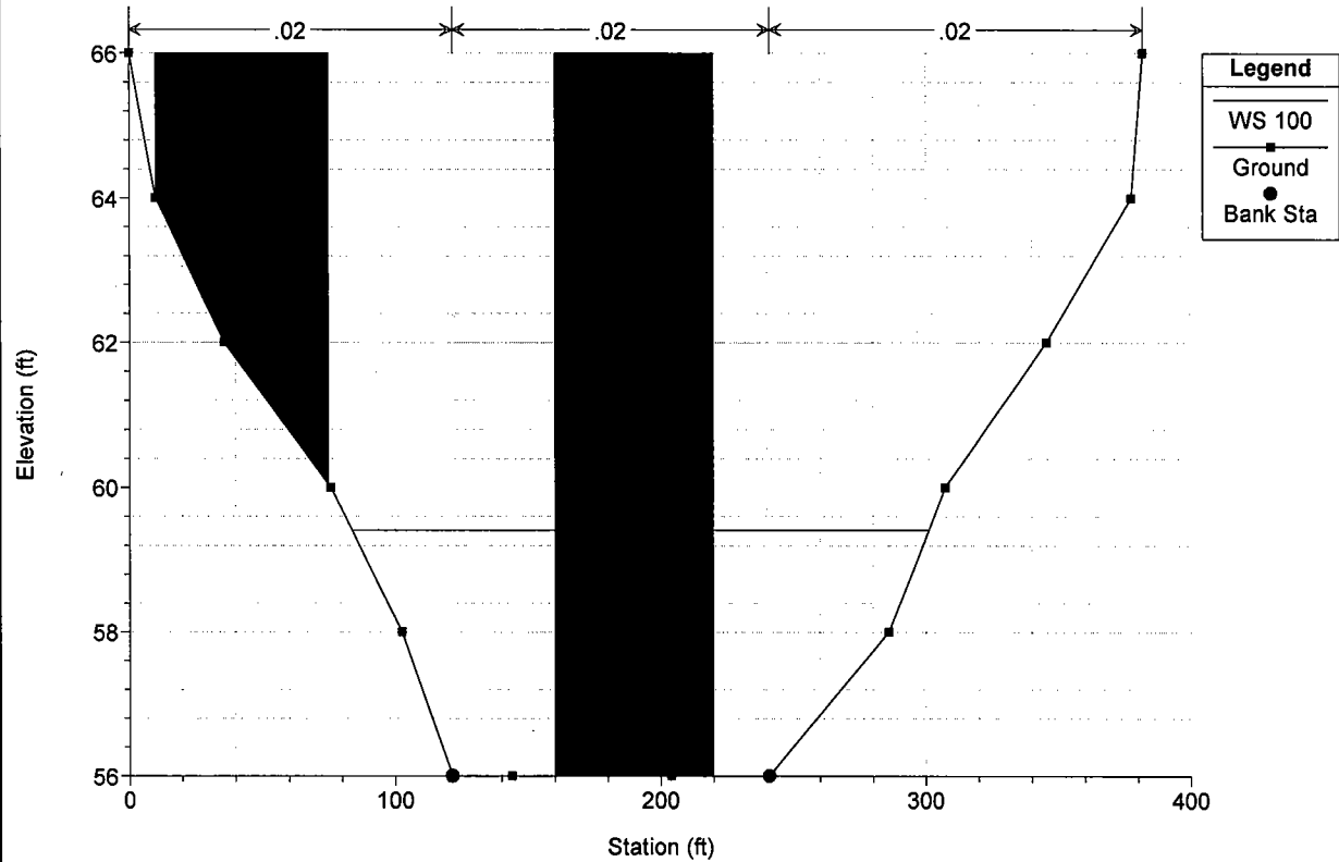
Encinitas Hwy 101 with Vulcan Plan: Alt 5 10-yr Cut River = Leucadia Reach = 101 RS = 215
