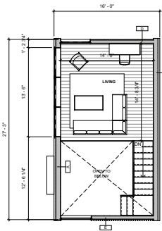
2 BUNGALOW B - ENLARGED FLOOR PLAN LOFT
